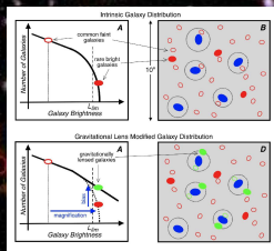
Fig. 2a. [Left]: Cartoon showing how magnification bias leads to an association between foreground galaxies and high redshift candidates. Fig. 2b. [Right]: Panel A: The Schechter LF of high redshift galaxies. Panel B: High redshift galaxies (red) and foreground galaxies (blue). Open symbols indicate undetected galaxies ( m_{AB} > m_{lim} ). Filled symbols are detected galaxies ( m_{AB} \leq m_{lim} ). Black dotted areas are regions of sky where background-sources will be multiply imaged by foreground galaxy halos (blue). Panel C: The lensed faint galaxies are multiply imaged, producing a detected image with m_{AB} \leq m_{lim} (green), and an undetected image with m_{AB} > m_{lim} (dotted green). Panel C: The resulting effect of gravitational lensing bias on z=8-10 galaxy samples. The observed LF can get modified from a Schechter function to a double power-law, with the brighter objects gravitationally lensed into the sample (Wyithe et al., 2011).
