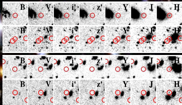
Fig. 3. [Above and Below]: Six examples of gravitationally lensed z=8-10 candidates behind foreground galaxies at z=1-2 (Yan et al. 2010) in the HUDF in BVIZ (ACS) YJH (WFC3). Until spectroscopic confirmation is available, these Y-band and J-band dropouts are only considered z=8 and z=10 candidates, resp. JWST will be essential to get spectra for such objects, especially for those z=8-10 candidates that are gravitationally lensed into the sample by z=1-2 foreground galaxies. (The background image of this poster also shows all available 506 orbits of the HUDF in the BVIZYJH filters (properly color balanced), with Y-drops or z=8 candidates marked as green circles, and I-drops or z=10 candidates as red circles. All Figures and Captions were placed to maximize the visibility of z=8-10 candidates.)
