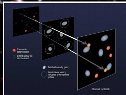
Fig. 2a. [Left]: Cartoon showing how magnification bias leads to an association between foreground galaxies and high redshift candidates. Fig. 2b. [Right]: Panel A: The Schechter LF of high redshift galaxies. Panel B: High redshift galaxies (red) and foreground galaxies (blue). Open symbols indicate undetected galaxies ( m_{AB} > m_{lim} ). Filled symbols are detected galaxies ( m_{AB} \leq m_{lim} ). Black dotted areas are regions of sky where background-sources will be multiply imaged by foreground galaxy halos (blue). Panel C: The lensed faint galaxies are multiply imaged, producing a detected image with m_{AB} \leq m_{lim} (green), and an undetected image with m_{AB} > m_{lim} (dotted green). Panel C: The resulting effect of gravitational lensing bias on z=8-10 galaxy samples. The observed LF can get modified from a Schechter function to a double power-law, with the brighter objects gravitationally lensed into the sample (Wyithe et al., 2011).
