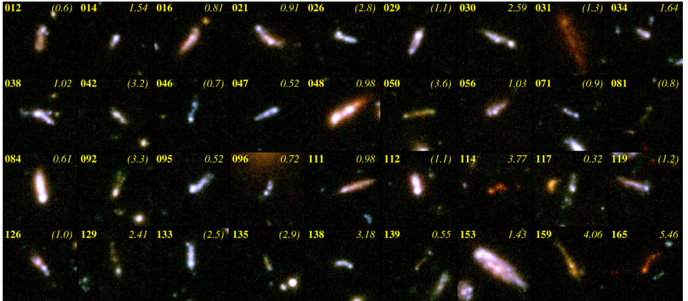
Fig. 1. i'_{AB} -Band mosaic of a subset of the HUDF tadpole galaxy sample. Stamps are 3 arcsec on a side. The vast majority of our tadpole sample contains the distinctive knot-plus-tail morphology.
