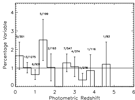
Fig. 7b. Percentage of HUDF objects to i_{AB} \lesssim 28.0 AB-mag showing variable point sources as a function of redshift. Within the statistical uncertainties, about 1% of all HUDF galaxies show point source variability over the redshift range surveyed ( 0 \lesssim z \lesssim 5 ). Hence, SMBH growth as traced by the weak AGN fraction keeps pace with galaxy assembly as traced by the tadpoles in Fig. 3b.
