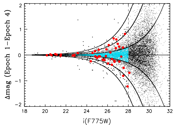
Fig. 4a. Magnitude difference between two HUDF epochs of all objects vs. i_{\text{AB}} -band flux from matched total apertures. The \pm 1\sigma , \pm 3\sigma , \pm 5\sigma lines are shown. Blue points show the |\Delta\text{mag}| \lesssim \pm 1.0\sigma points used to normalize the error distribution. Large red points show the “best” 45 variable candidates from all six possible epoch combinations, many of which were seen at \gtrsim 3.0\sigma in two or more epoch combinations.
