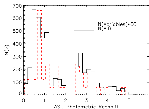
Fig. 7a. Photometric redshift distribution of all HUDF field galaxies to i'_{\text{AB}} \lesssim 28.0 mag (solid line), and for the “best” variable candidates (red dashed line) multiplied by 60\times for best comparison. The redshift distribution of the variable objects follows that of field galaxies in general (For interpretation of the references to color in this figure legend, the reader is referred to the web version of this article.).
