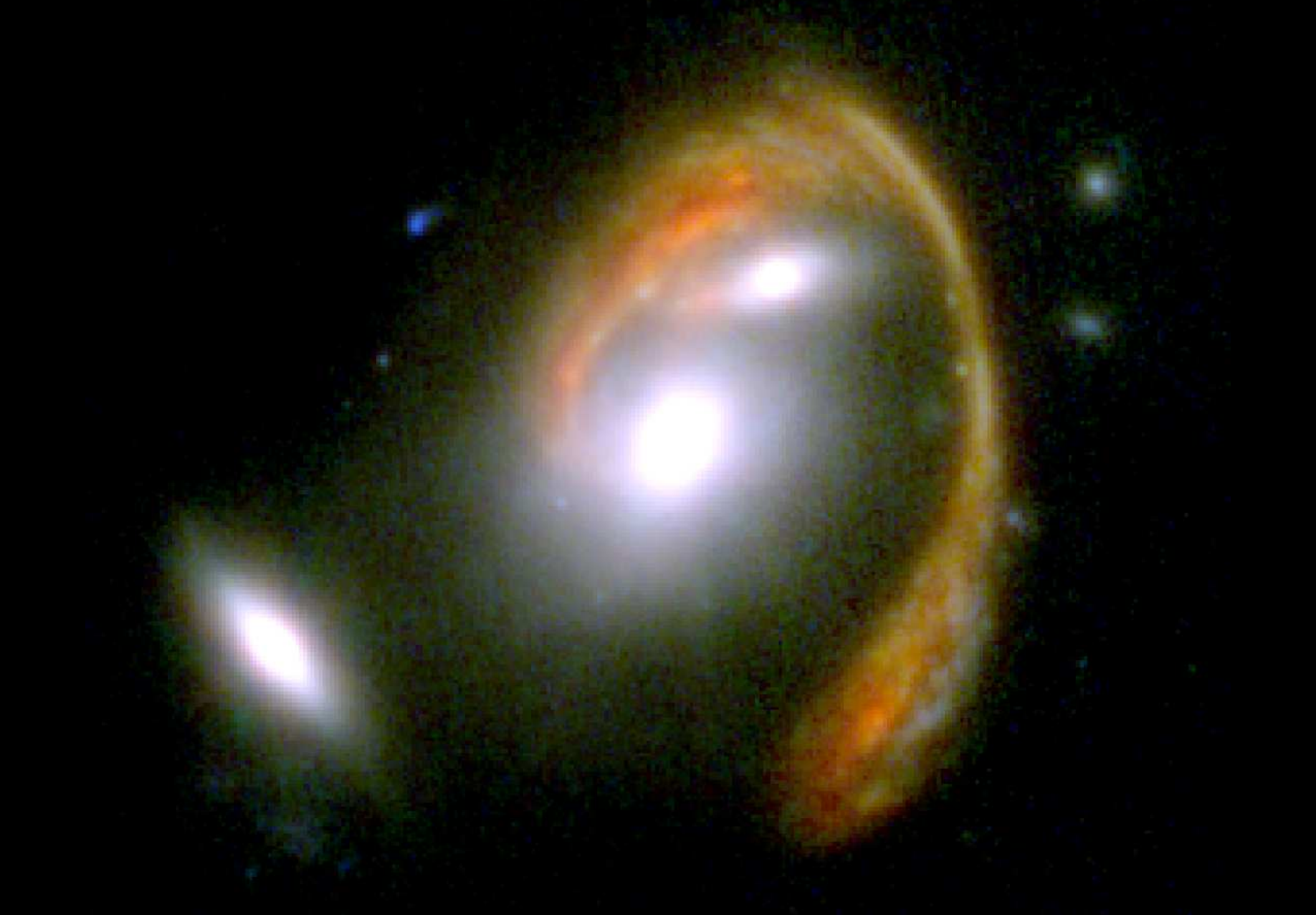
and El Gordo makes a super-lens “El Anzuelo” — Einstein’s fishhook!
